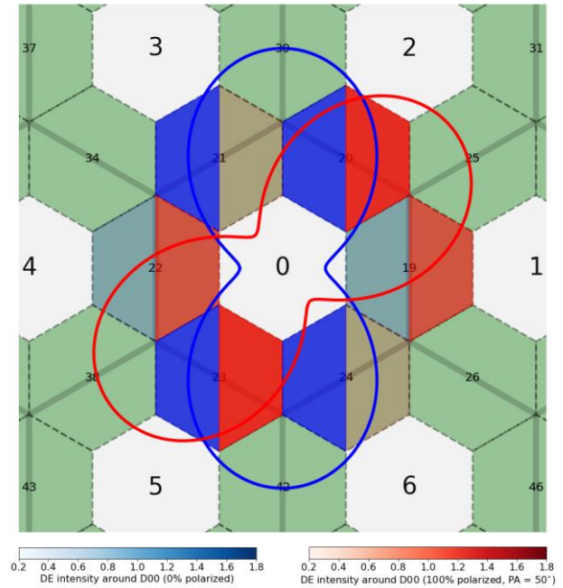
Figure 8: SPI detector array (numbered hexagons) and the differential Klein-Nishina cross-section (red/blue).
