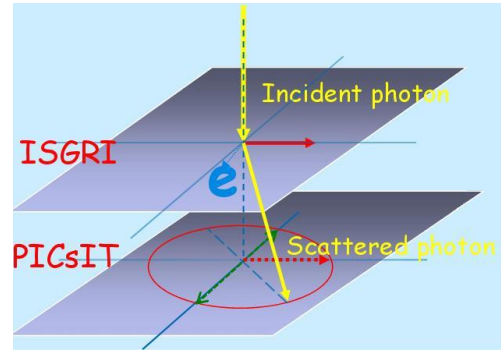
Figure 9: Schematics of the Compton scattering between the two IBIS sub-detectors ISGRI and PICsIT [From Laurent 2017, talk at Hiroshima Conf., Feb. 2017].
